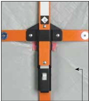
Single Trigger Release The patented MDI Compact Collapse & Wrap sign system features signs that have hinged, integrated crossbracing with a single trigger release mechanism for rapid deployment and take-down.
