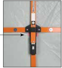
Single Trigger Release The patented MDI Compact Collapse & Wrap sign system features signs that have hinged, integrated crossbracing with a single trigger release mechanism for rapid deployment and take-down.
